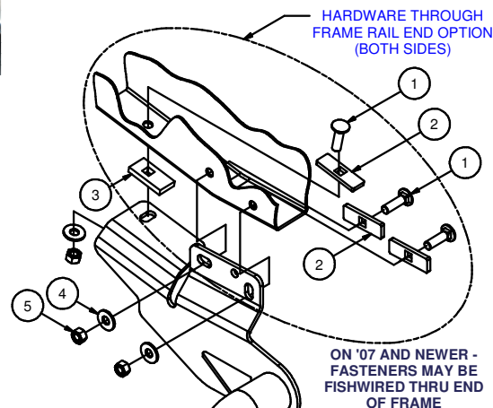
EXHAUST DAMPENER
